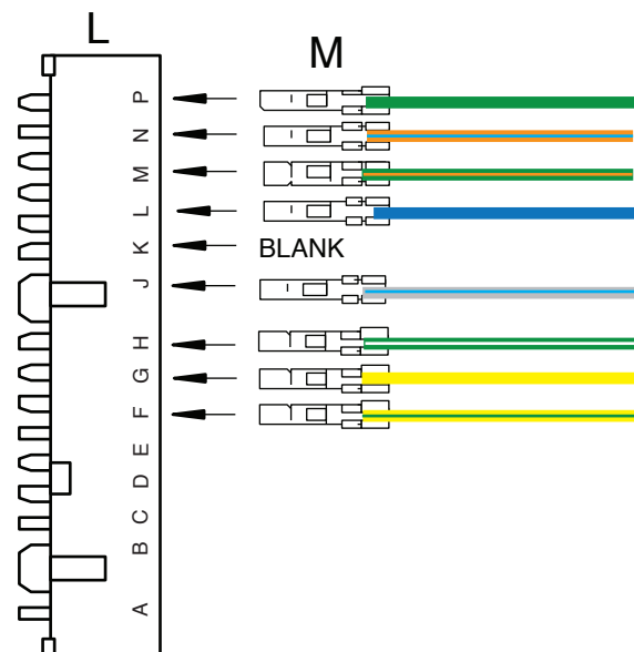
DIAGRAM 'A' - AAW Turn Signal Switch Wires to Stock 1965 Steering Columns.
