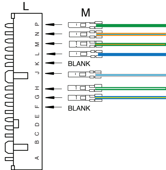
DIAGRAM 'A' - AAW Turn Signal Switch Wires to Stock 1960-64 Steering Columns.
